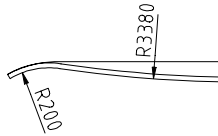
SECTION 1-1
